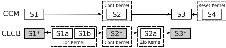
Fig. 1. The CCM and CLCB algorithms compared
