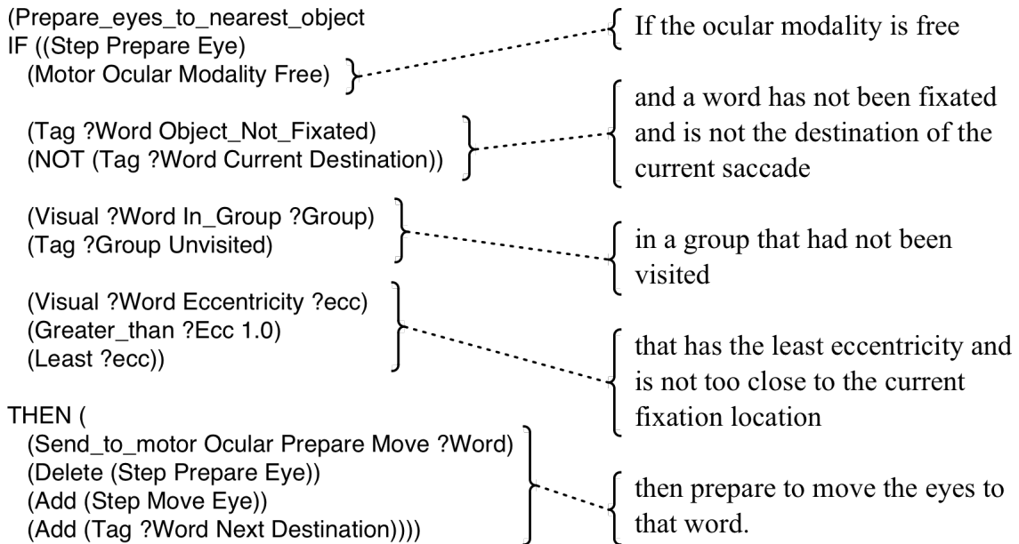
Figure 2. Example EPIC production rule that illustrates the selection of a saccade destination and prepares an eye movement to that location.
