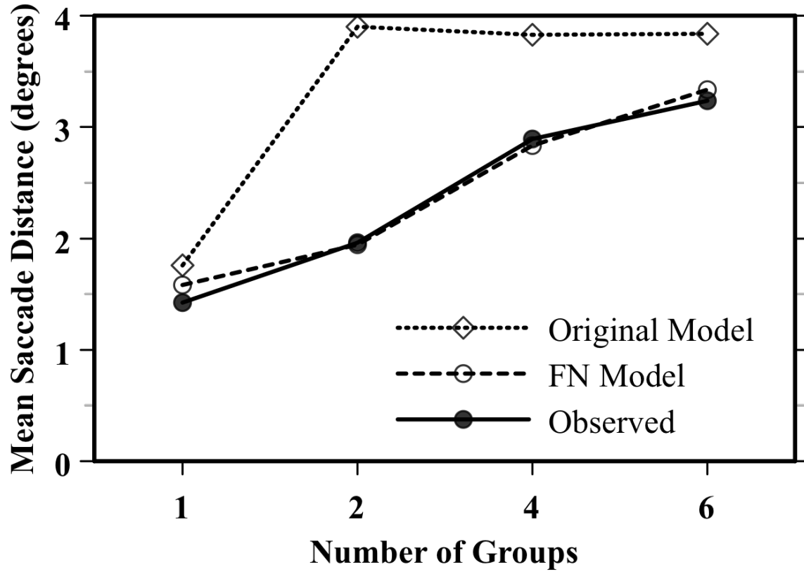
Figure 8. Saccade distance observed in the CVC search task, predicted by the original CVC search task model and predicted by the fixate-Nearby (FN) Model. The AAE of the original model is 43.3% and of the FN model is 4.2%.
