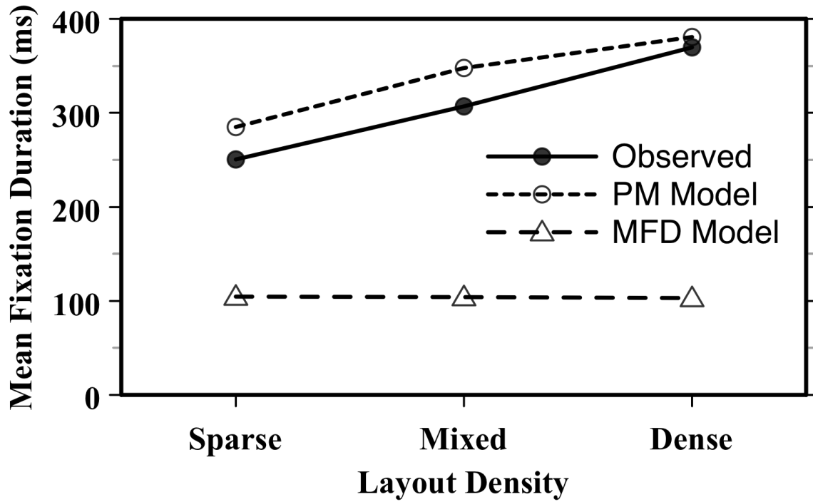
Figure 5. Mean fixation durations observed and predicted by the process-monitoring model (PM) and minimum fixation duration model (MFD) for the mixed density task. The average absolute error (AAE) of the PM model is 10.0% and the MFD model is 65.5%.
