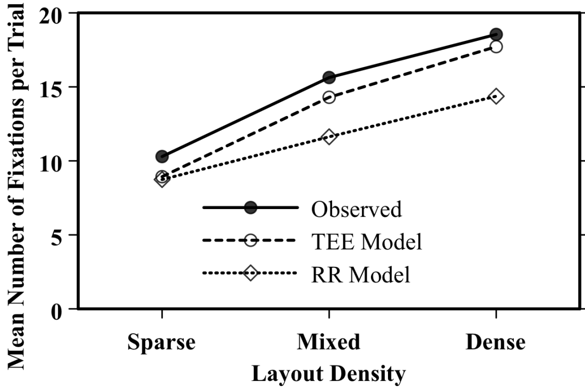
Figure 7. Mean number of fixations per trial observed, predicted by the Text-Encoding Error (TEE) model and the Reduced-Region (RR) model for the mixed-density task. The AAE of the TEE model is 8.8% and the RR model is 21.1%.
