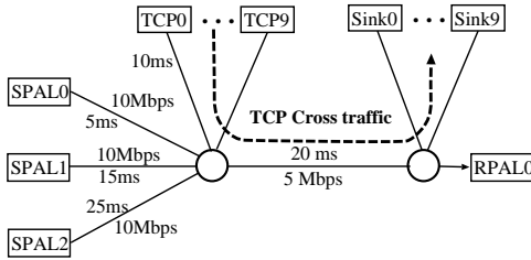
Figure 5: Simulation Setup
