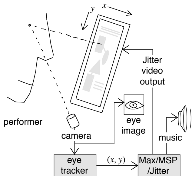
Figure 1. The EyeMusic system architecture. Arrows indicate the flow of data.
