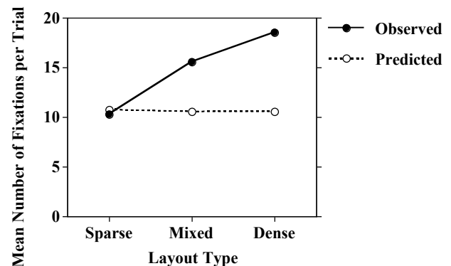
Figure 3. Mean number of fixations per trial observed (solid line) and predicted (dashed line) by the purely random base model. AAE = 26.7%
