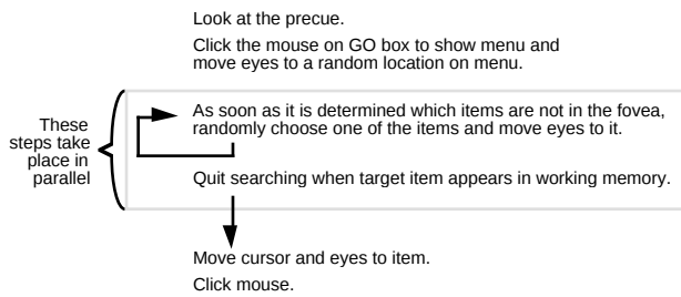
Figure 7. Parallel Processing Random Search model.
