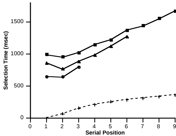
Figure 3. Nilsen's observed data (solid lines). Mean selection times as a function of serial position of target item, for menus with three, six, or nine items. Also: Time required to move the mouse to each target position as predicted by Fitts' law (dashed line).
