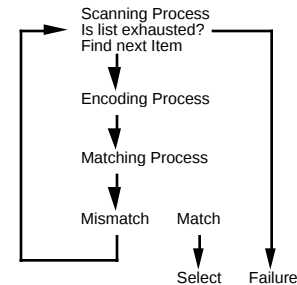
Figure 4. Norman's [12] information processing model for search of an explicitly known target.
