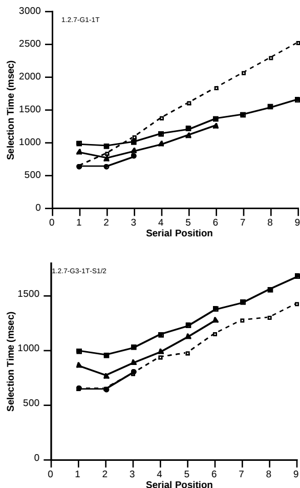
Figure 10. Selection times observed (solid lines) and predicted (dashed lines) by the Parallel Processing Systematic Search model run with one item (top graph) and three items (bottom graph) fitting into the fovea. In each graph, the predicted times for the same serial position in different length menus are the same and are thus superimposed.
