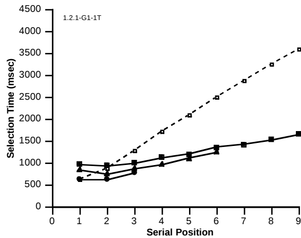
Figure 6. Selection times observed (solid lines) and predicted (dashed lines) by the Serial Processing Systematic Search model run with one item fitting into the fovea. The predicted times for the same serial position in different menu lengths are the same and are thus superimposed.
