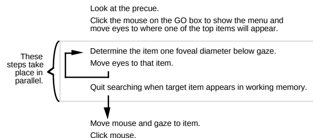
Figure 9. Parallel Processing Systematic Search model.
