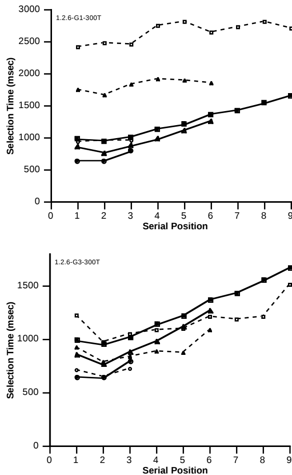
Figure 8. Selection times observed (solid lines) and predicted (dashed lines) by the Parallel Processing Random Search model run with one item (top graph) and three items (bottom graph) fitting into the fovea.
