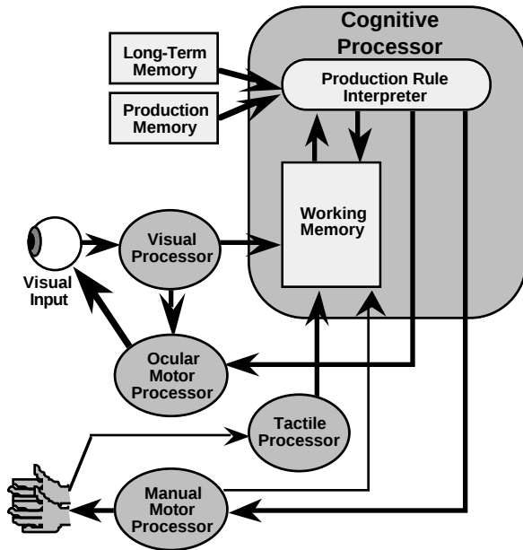
Figure 1. Subset of EPIC architecture, showing flow of information and control. The processors run independently and in parallel. Not shown: Auditory and vocal motor processors, task environment.
