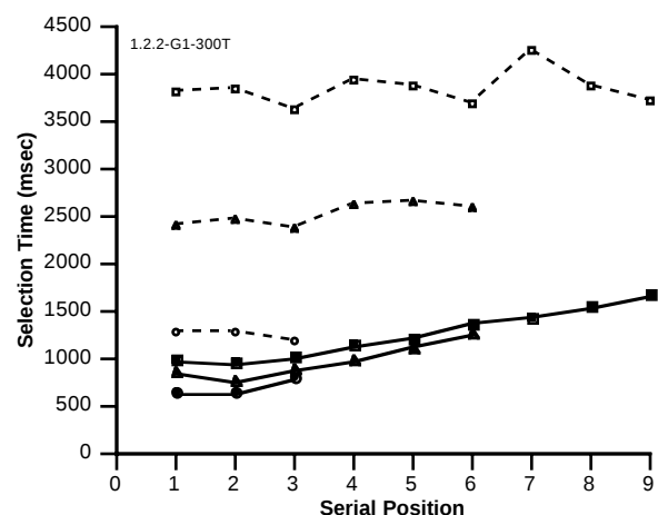
Figure 5. Selection times observed (solid lines) and predicted (dashed lines) by the Serial Processing Random Search model run with one item fitting into the fovea.
