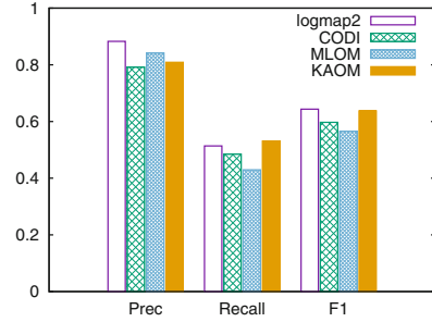
Fig. 2. Precision, recall and F1 on the OntoFarm domain with only the one-to-one correspondences.
