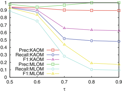
Fig. 1. Precision, recall and F1 on the census domain as a function of the string similarity threshold \tau .
