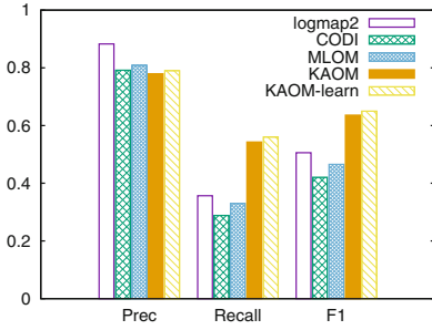
Fig. 3. Precision, recall and F1 on the OntoFarm domain with the complex correspondences.
