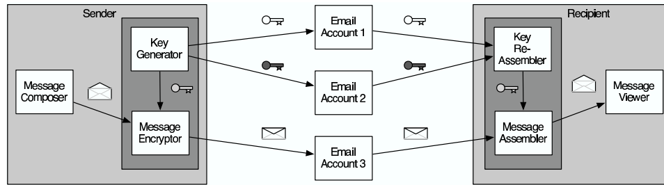
Fig. 1.1. A sample message and key delivery flow. The sender encrypts the plaintext and then embeds it into carefully select coverttext using steganography. The message containing the hidden content is then sent as shares to one or more accounts owned by the recipient. Each of the key shares used to create the encryption key are then sent to different destination email accounts. The recipient's client checks all of the accounts, reassembles the key and ciphertext from the shares, and recovers the plaintext. The separate emails from different SMTP servers to prevent reassembly by adversaries.
